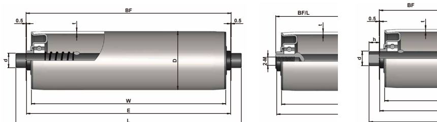
Spring loaded
