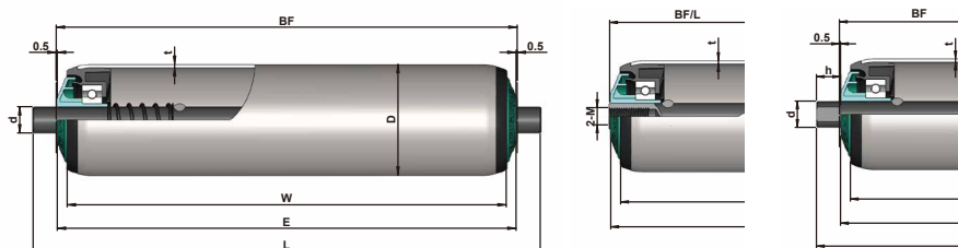
Spring loaded
